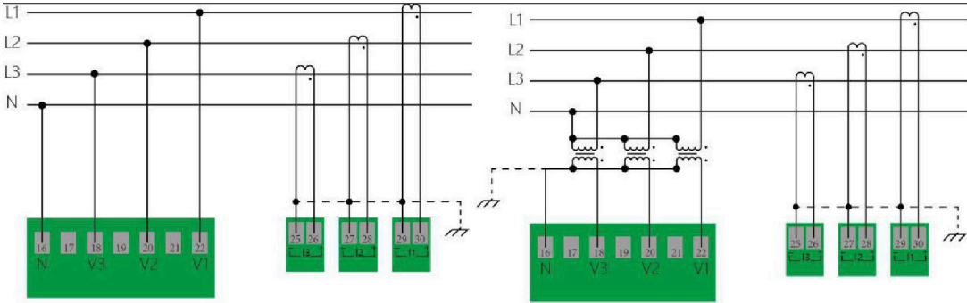
3PH4W (without PT) wiring diagram
