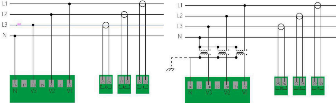
3PH4W (without PT) wiring diagram
