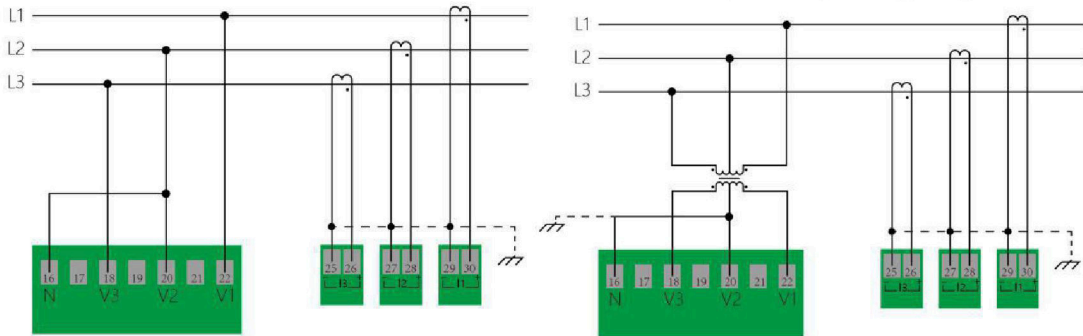
3PH3W (with PT) wiring diagram
