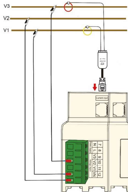
Three-phase three-wire2CT
