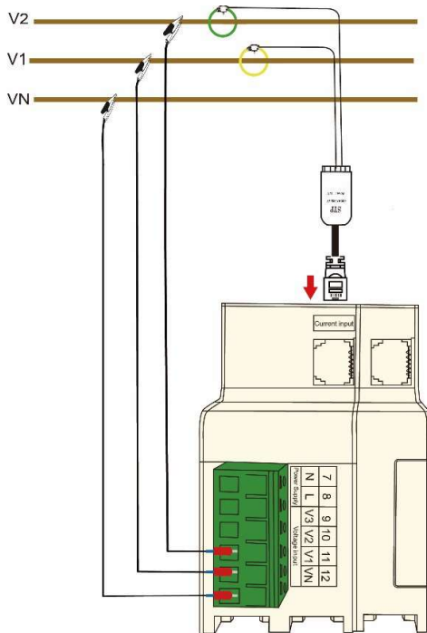
One-phase three-wire
